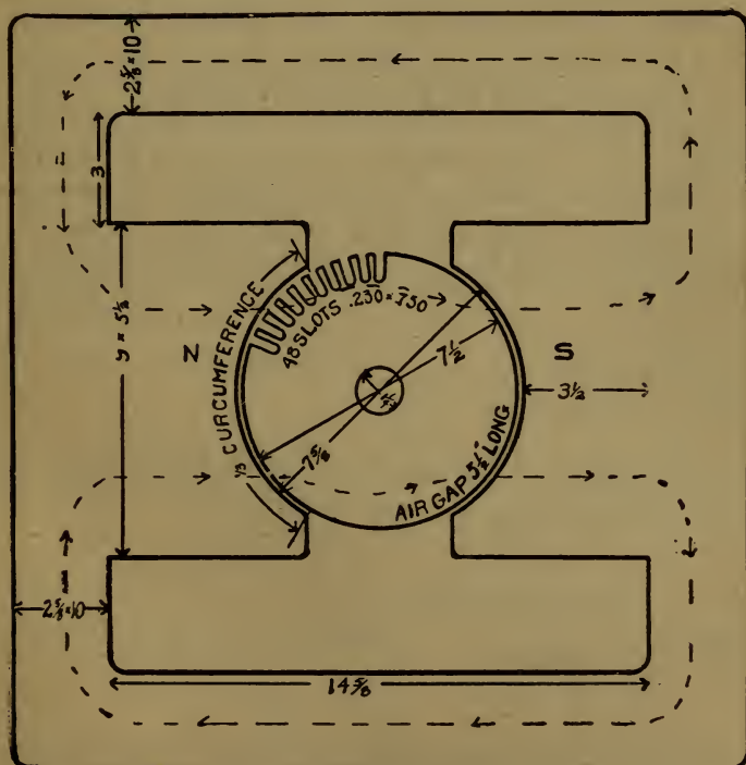
Figure 31 Magnetic circuit of 5 H. P. bipolar machine with iron clad armature, and cast iron field frame.
